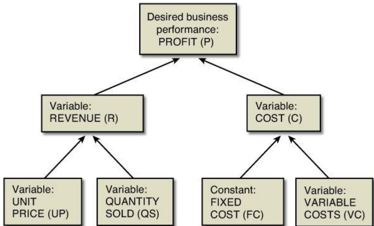
Figure 6.2 An influence diagram
